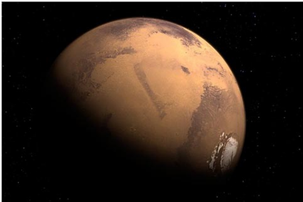
Mars Polar Ice from Orbit
